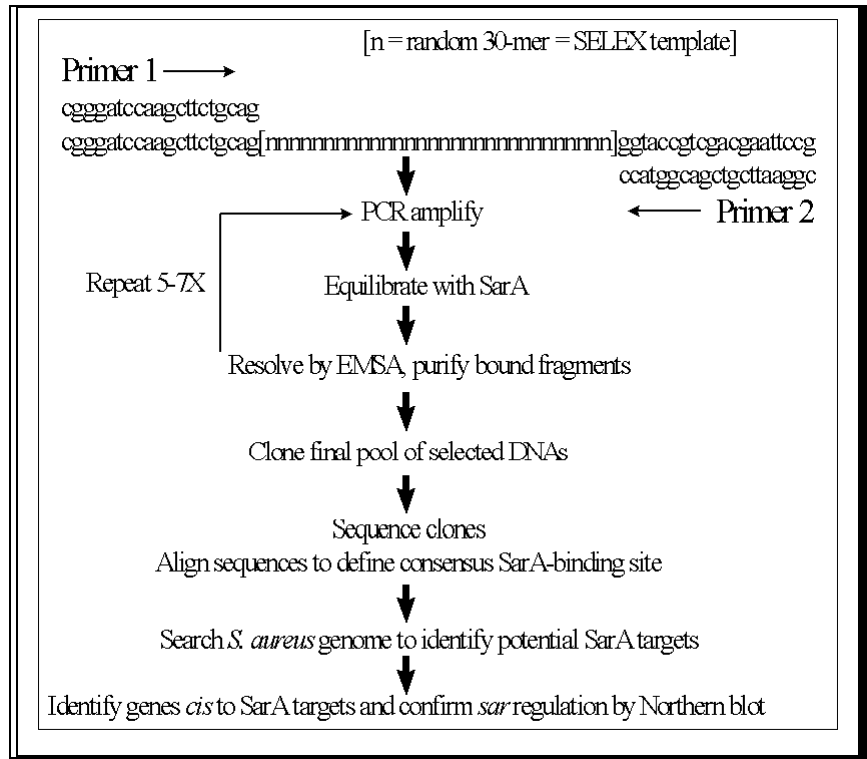
Fig. 14. Flow-chart for PCR-assisted binding site selection (PCR-ABS).
